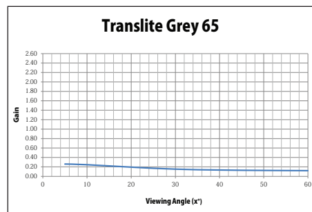
Screen Gain
