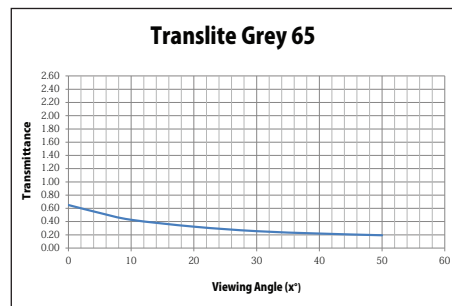
Screen Transmittance
