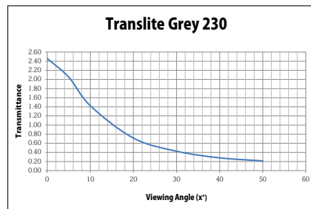
Screen Transmittance
